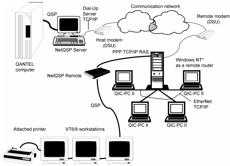
Remote Site with Windows NT
