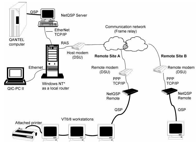
Multiple Remote Sites
